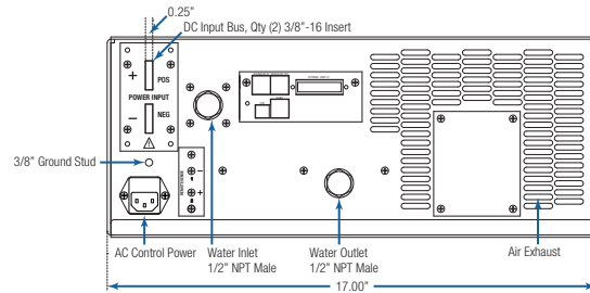
WRx Series 12.5 kW, Rear View
