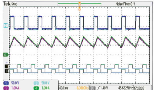
Ultra-high fidelity: magenta: real boost MPPT converter current; green: HIL boost current; dark blue: real boost inductor voltage; light blue: HIL inductor voltage.
